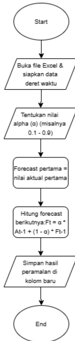
Gambar. 3.3 flowchart metode exponential smoothing
