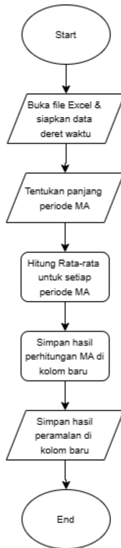
Gambar 3. 2 Flowchart Metode Moving Average
