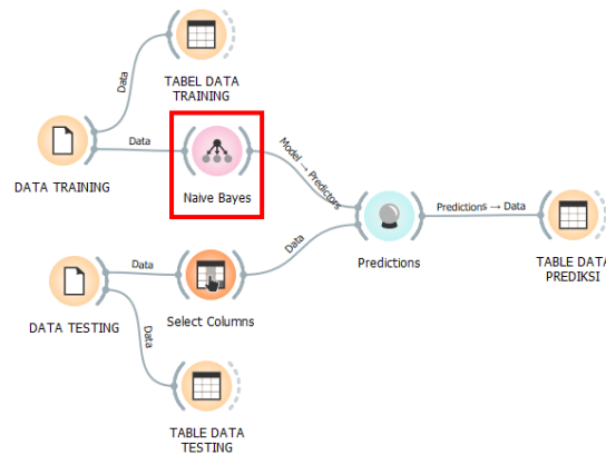
Fig 3. Classification Process in Data Mining
