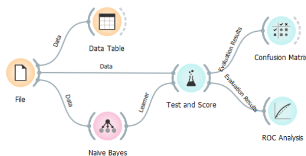
Fig 4. Design Widget Evaluation Process
