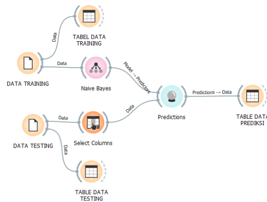
Fig 2. System Design Process in Data Mining
