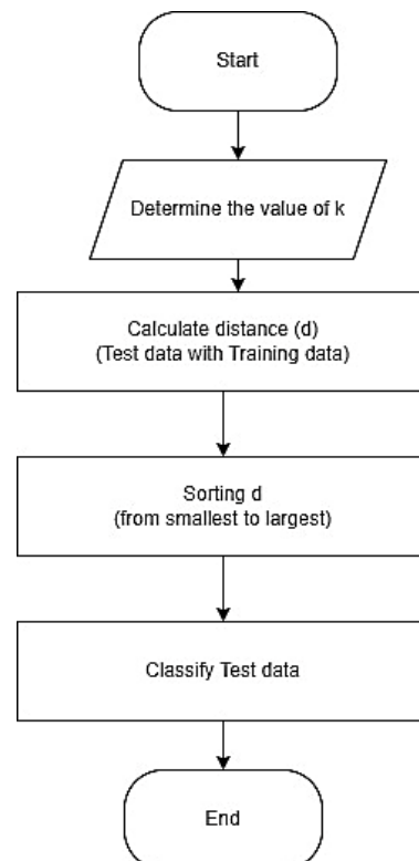
Figure 3. k-NN Algorithm flowchart
