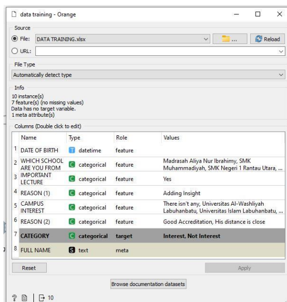
Figure 1. Selection of training data targets
