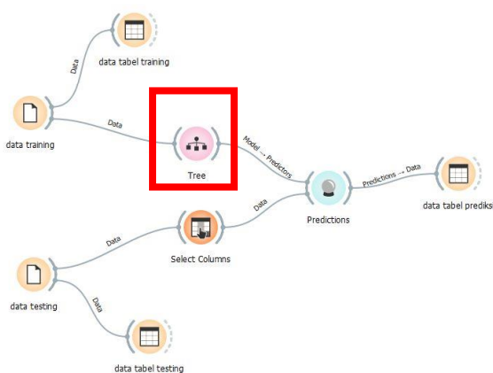
Figure 4. Widget design model classification of scholarship acceptance status dataset
